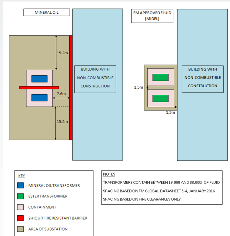
Figure 1 - Example installations, mineral oil and FM Approved fluid
